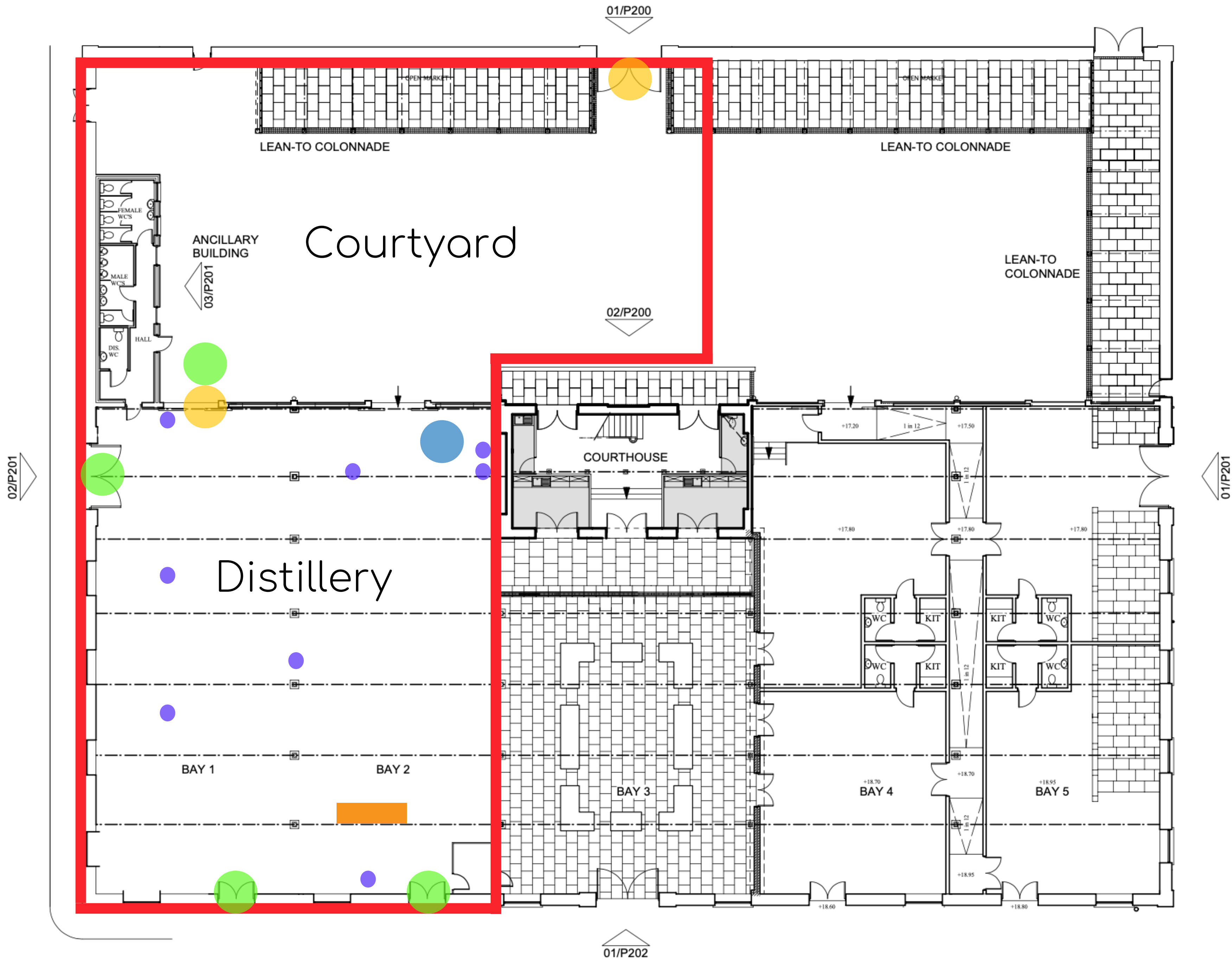
01. GROUND FLOOR PLAN 1:200
